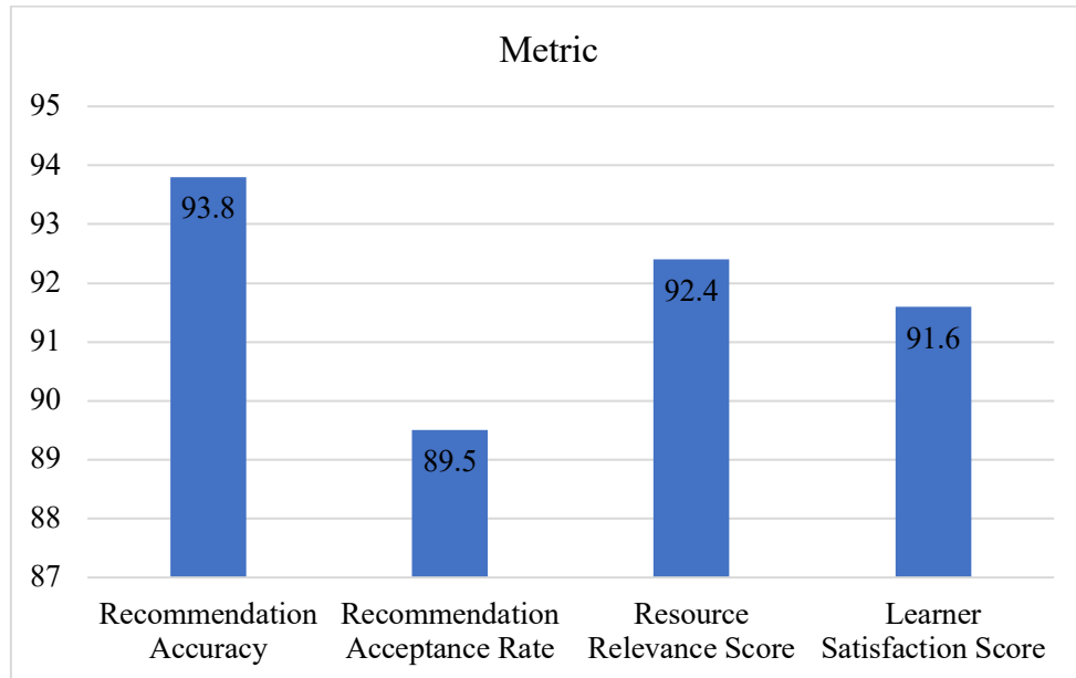
Figure 3. Recommendation Performance
