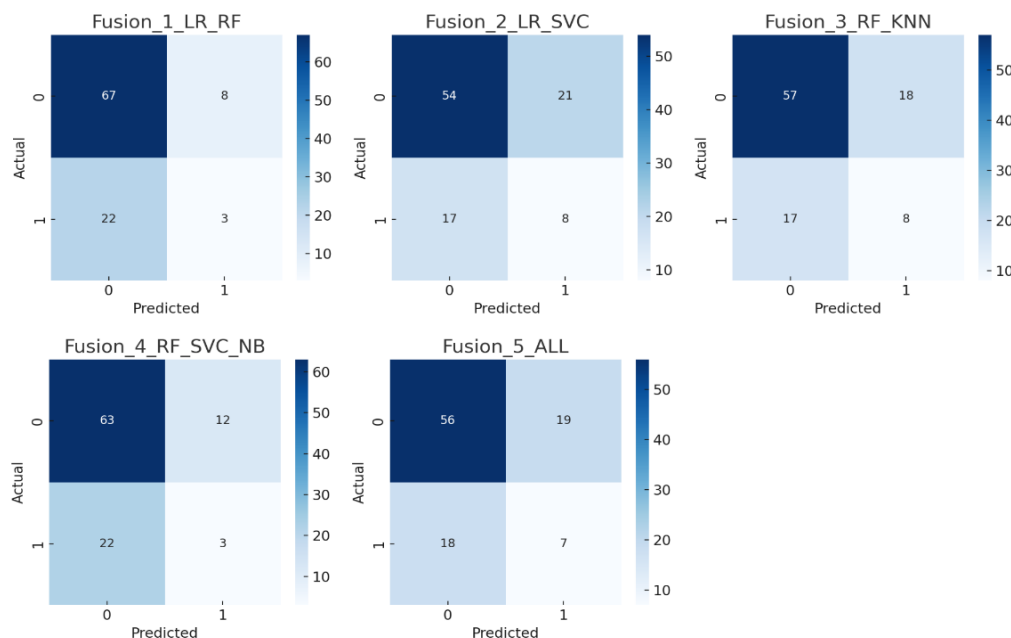
Figure 3. Confusion Matrices for Five Fusion Configurations.
