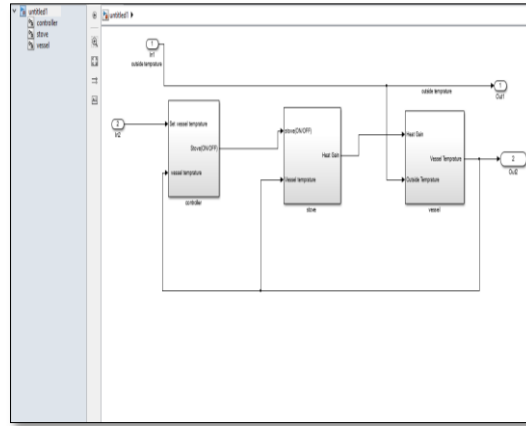
Figure 4. Simulink model to control stove
