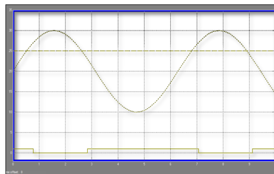
Figure 5. Temperature variations
