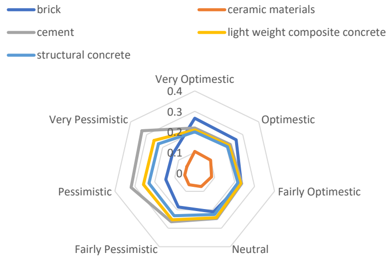
Figure 10. The outcomes of the OWA method on different WTS applications
