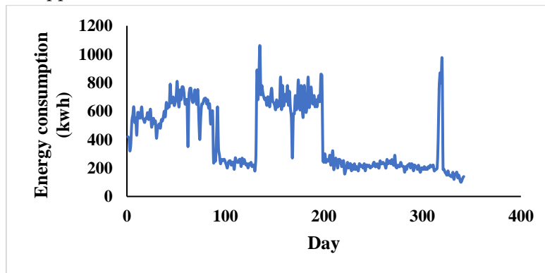
Figure 6. The Energy consumption of coagulation and flocculation unit per day in WTP's No. 1
