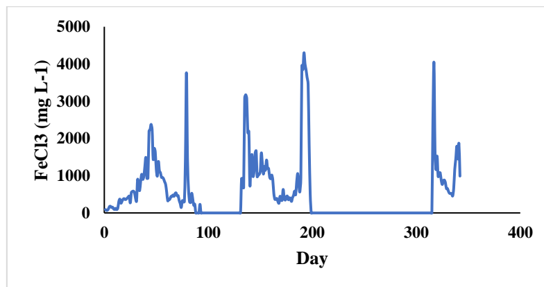
Figure 7. The amount of \text{FeCl}_3 per day in WTP's No. 1, Mashhad, Iran
