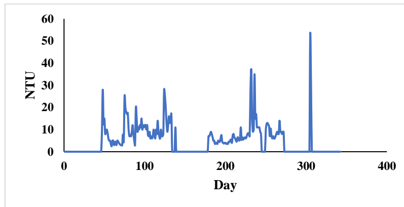
Figure 8. The fluctuation of influent TU per day in WTP's No. 1, Mashhad, Iran
